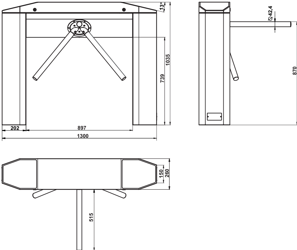
Dimensional Diagram
